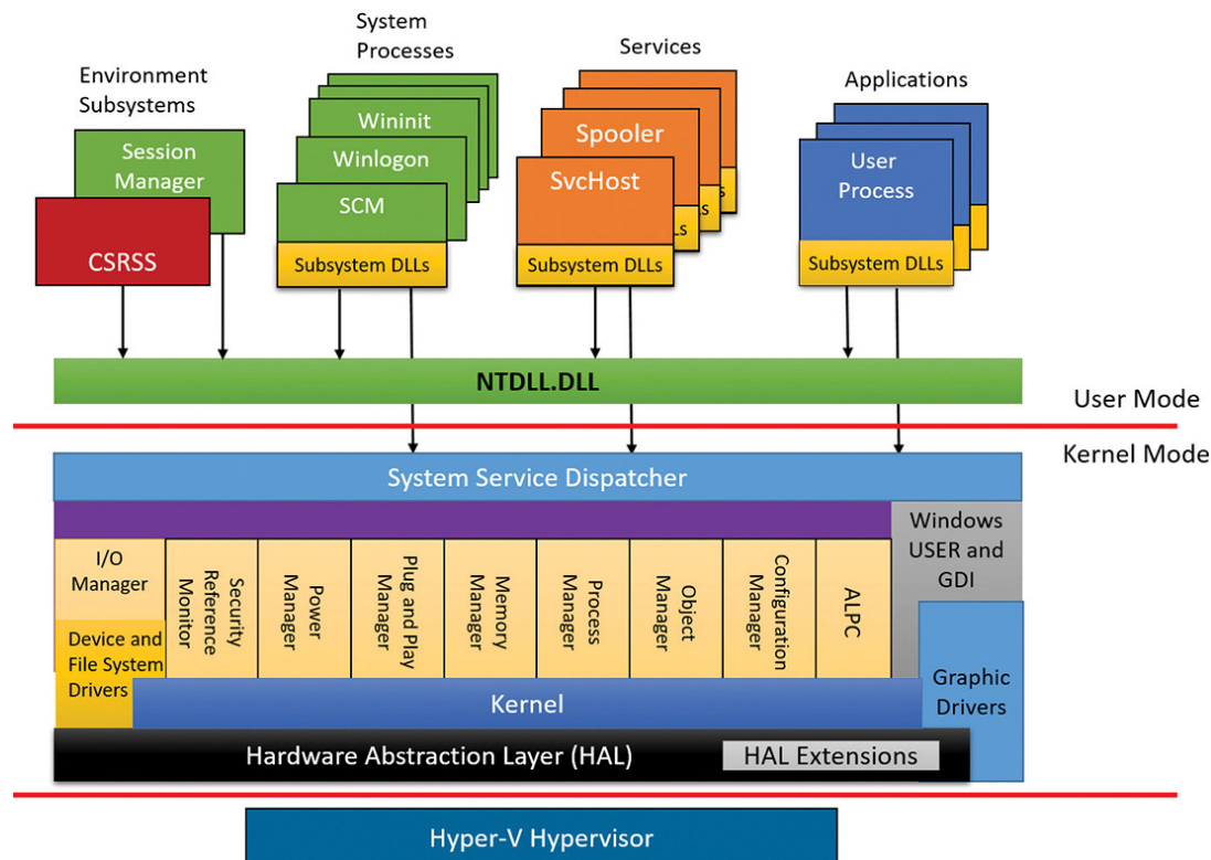
FIGURE 2-4 Windows architecture.
